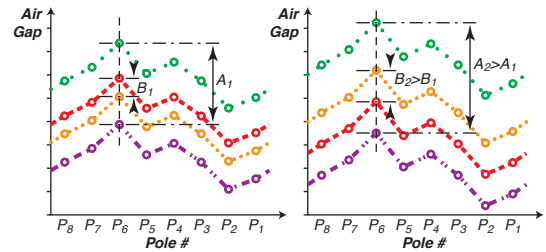
Figure 11: Comparison of Signature measurement graphs at two operating conditions: variations between two points from one graph to another are not the same; order of curve appearance can change.
