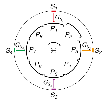
Figure 1: Example of a theoretically perfect generator with a round rotor inside a round stator. Pole [P_2] is deliberately protruding for comparison below.
