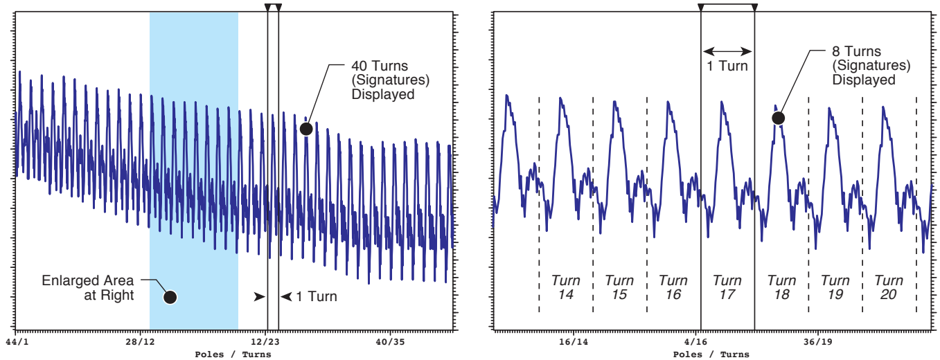
Figure 4: Graphs of Pole measurement showing parameter evolution over multiple turns. One can see the variation of rotor circularity, vibration amplitude, and patterns.
