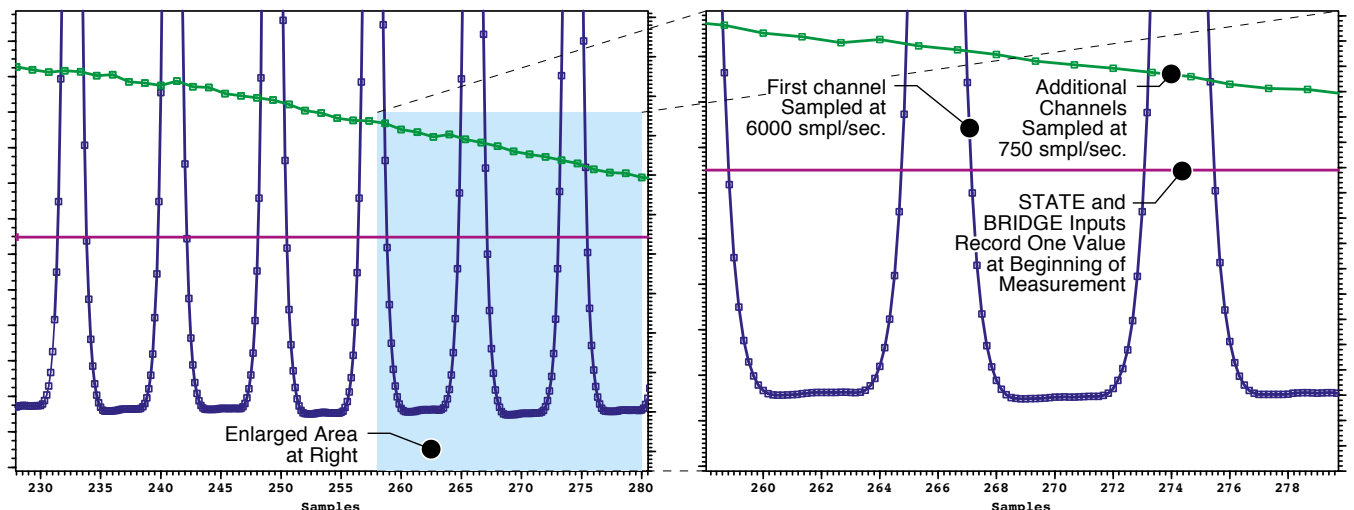
Figure 2: Graphs of Sampling measurement. Data is recorded at full sampling rate (6000 samples/sec. on Channel #1, 750 samples/sec. on additional channels, 1 value per measurement for STATE and BRIDGE inputs).
