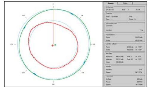
Generator Air Gap Polar Graph
