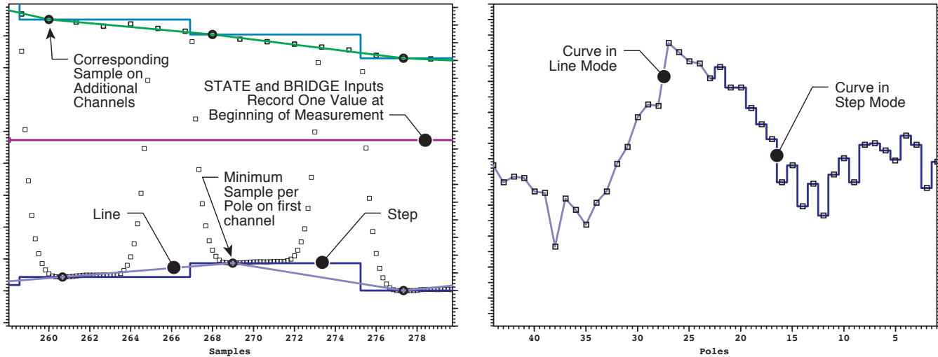
Figure 3: Graphs of Signature measurement. Each acquisition unit retains the minimum sample per pole on Channel #1 and corresponding samples for additional channels over one machine rotation. The graph at right shows the difference between curves traced in Line and Step modes.
