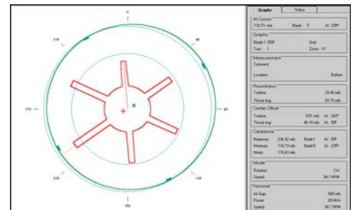
Turbine Blade Tip Clearance Polar Graph
