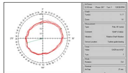
Shaft Orbit Graph
