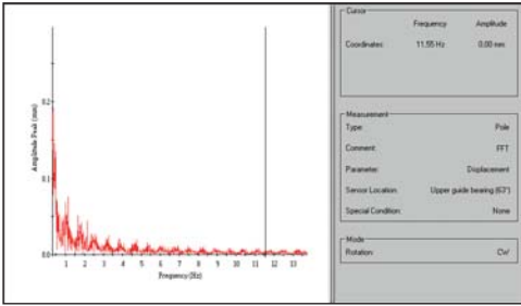
Spectrum Graph from ZOOM Analyst software
