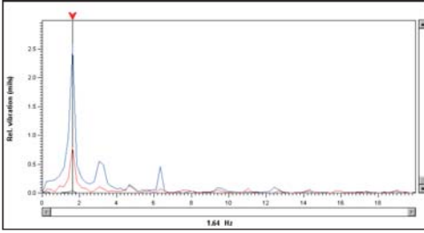
Spectrum Graph from ZOOM Application software
